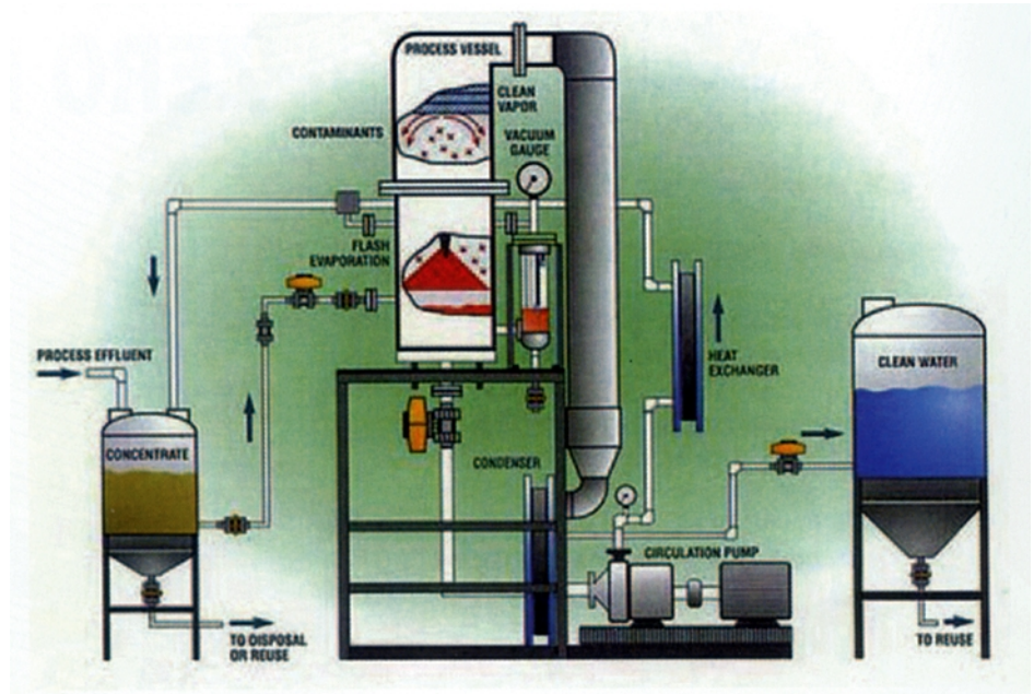
Diagram of the CASTion zero-discharge flash distillation system installed at Columbia Manufacturing.
